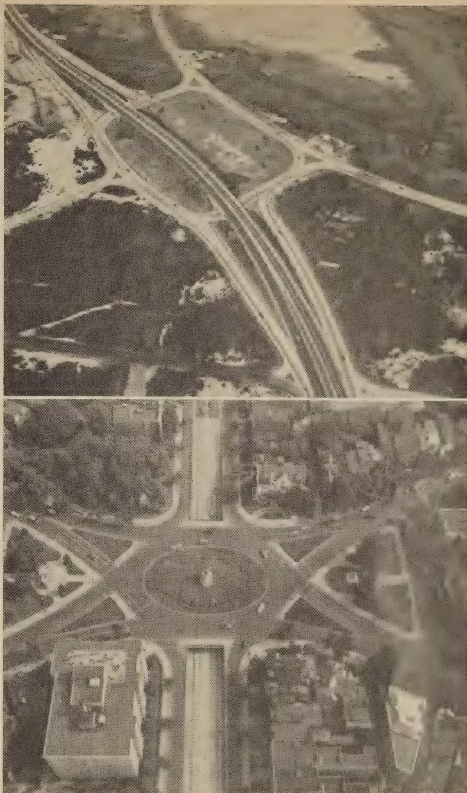
Traffic circles take many forms: Shown here are tangent and circular sections for weaving. When traffic circles are no longer able to accommodate their traffic loads the necessary remedial measures, such as an added overpass (above) or tunnel (below), may cost several million dollars.
